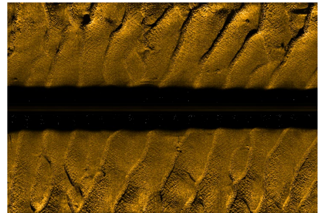
4K-UHR – Sand waves and Targets
